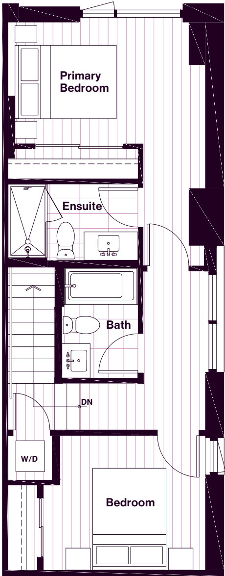
LEVEL 2
