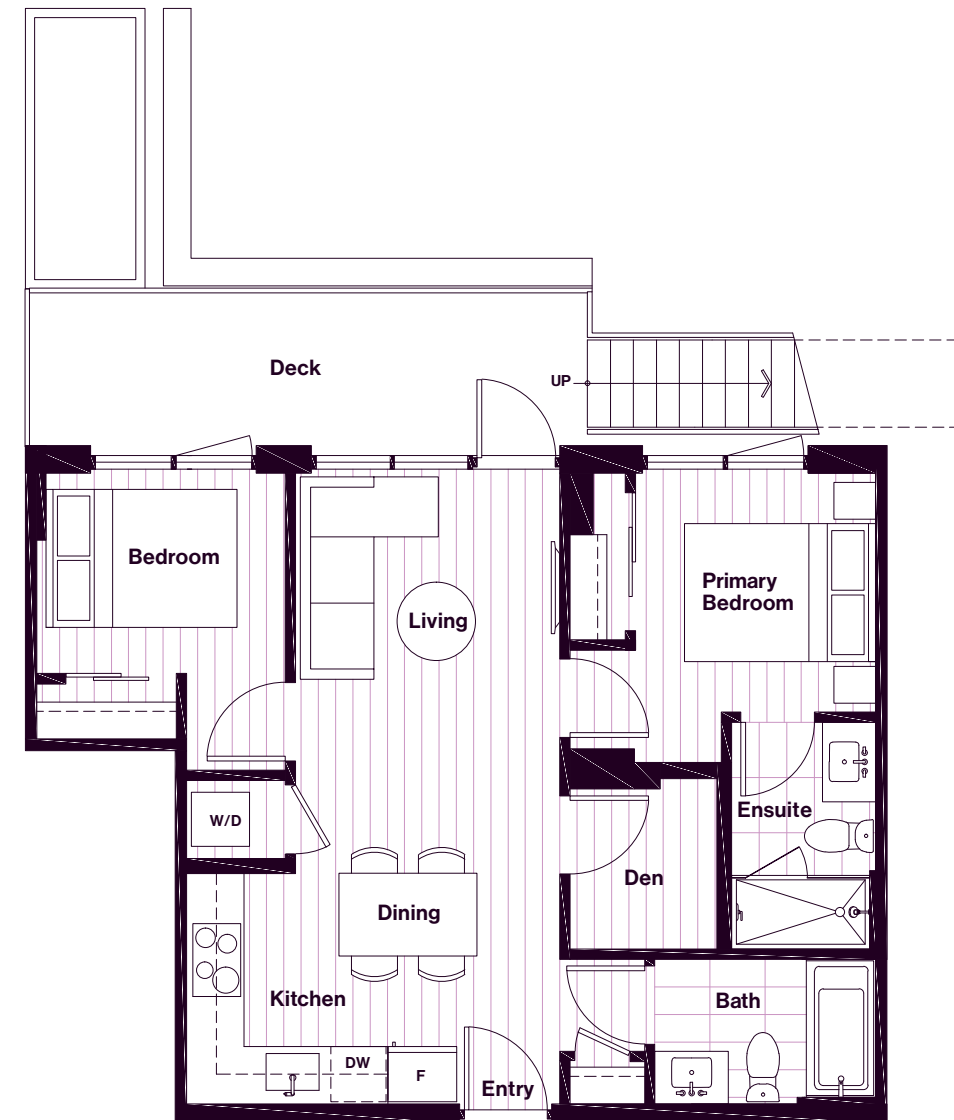
LEVEL 6
