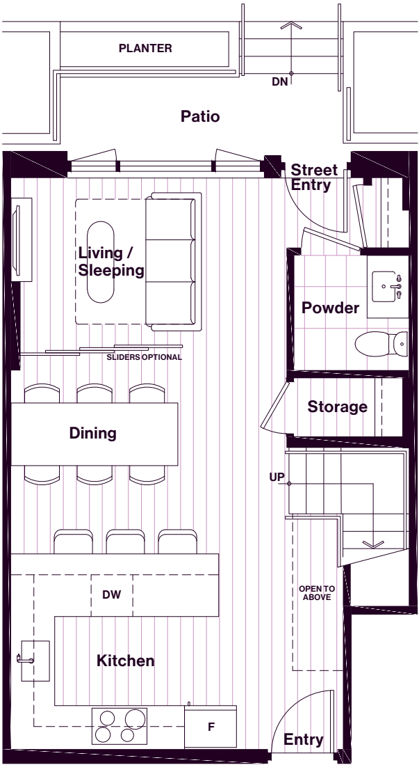
LEVEL 1
