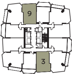
FLOORS 10 - 12, 17
